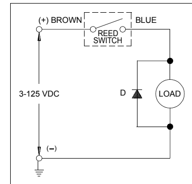
LOAD MUST NOT EXCEED 5 WATT SWITCH RATING D = DIODE MATCHED TO LOAD VOLTAGE & CURRENT
