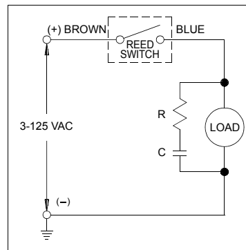
LOAD MUST NOT EXCEED 5 WATT SWITCH RATING R = RESISTOR (Under 1k OHM) C = CAPACITOR (0.01 Microfarad)
