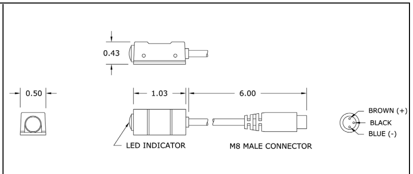
Pigtail Connection Type w/Bands
